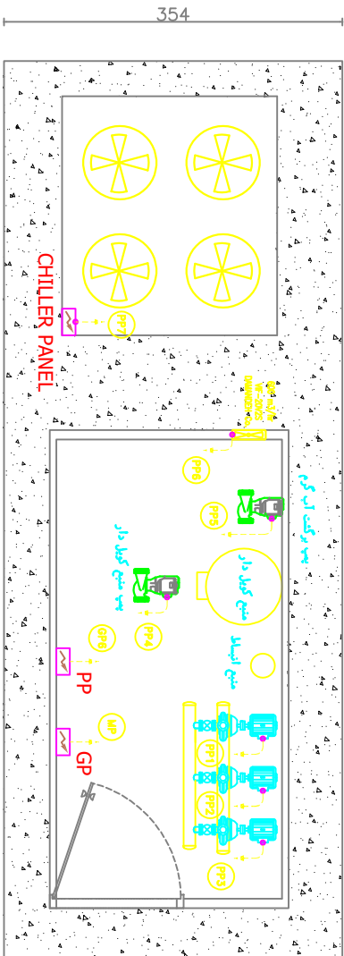
PUMP STATION POWER LAYOUT
