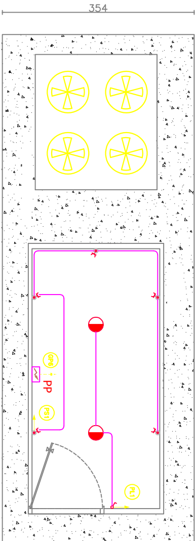
LIGHTING AND SOCKET LAYOUT
